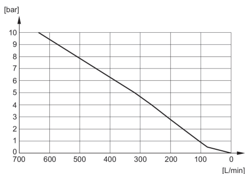
Flow diagram 1827000018
