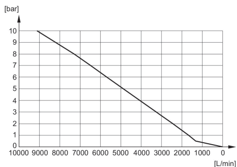
Flow diagram 1827000021
