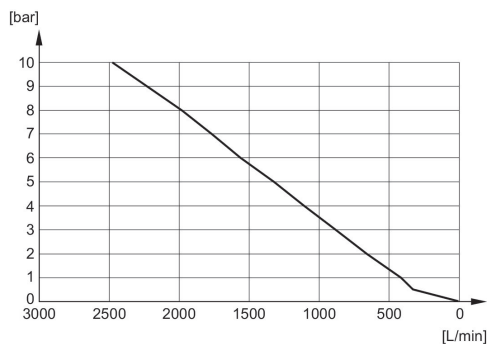
Flow diagram 1827000019
