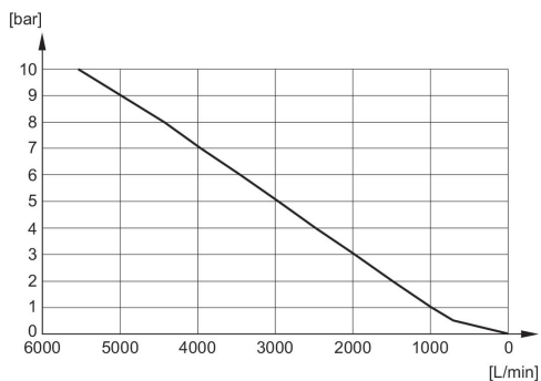
Flow diagram 1827000020
