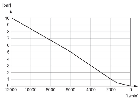
Flow diagram 1827000022
