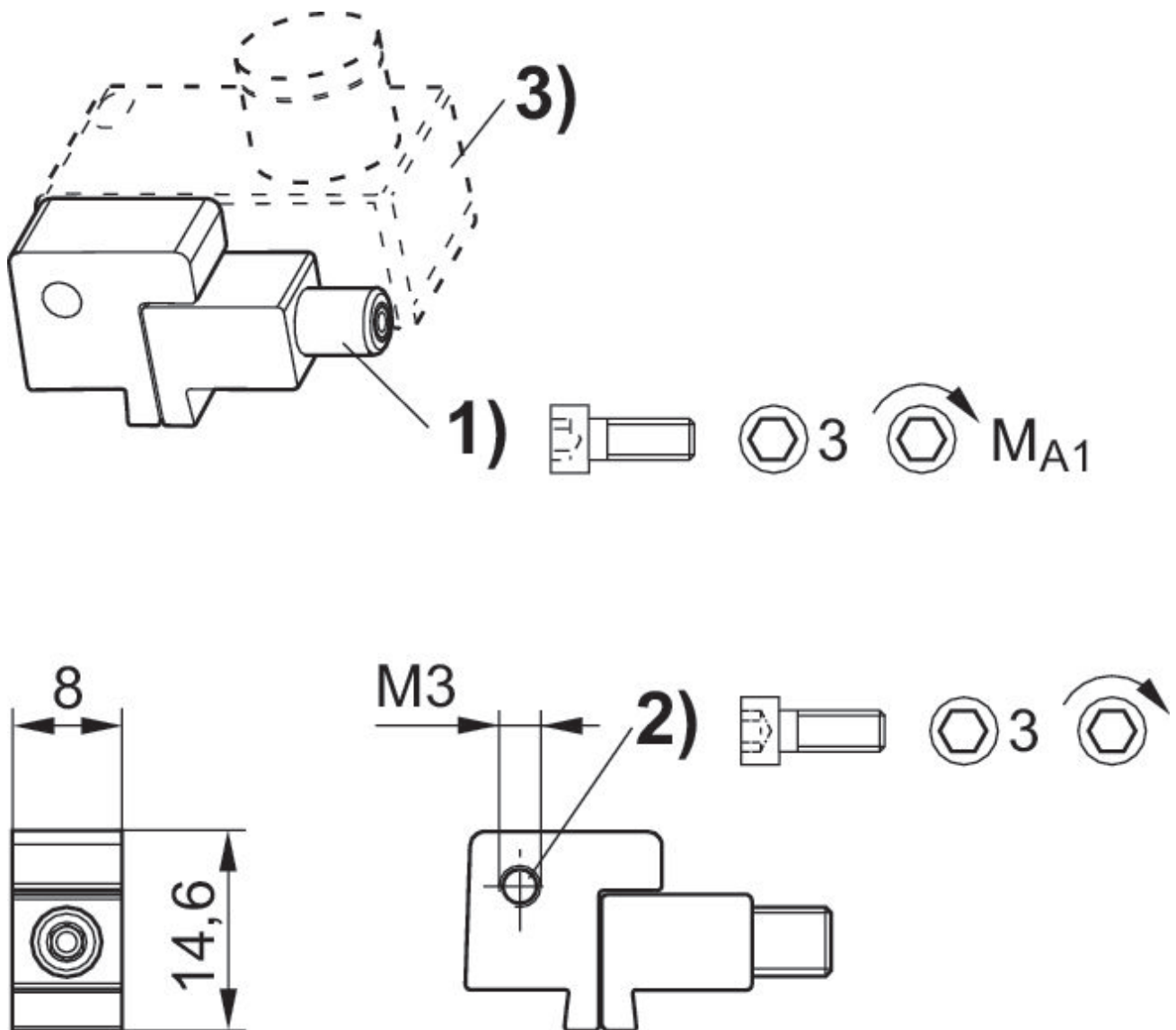
1) Clamping screw 2) Mounting screw for sensor 3) Sensor
