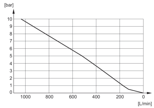
Flow diagram R412000591
