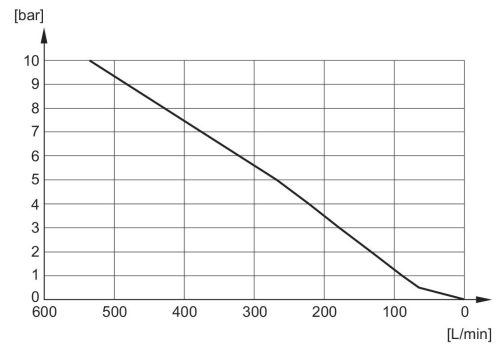
Flow diagram R412007519
