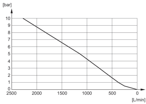
Flow diagram R412007520
