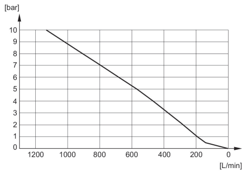
Flow diagram R412007899
