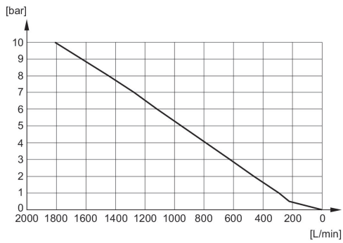
Flow diagram 1827000033
