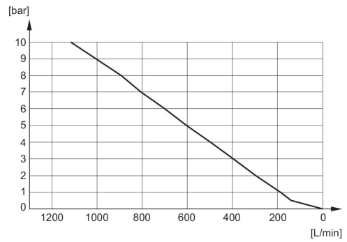
Flow diagram 1827000031
