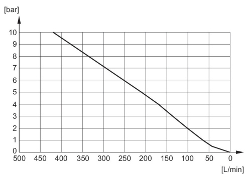
Flow diagram 1827000032
