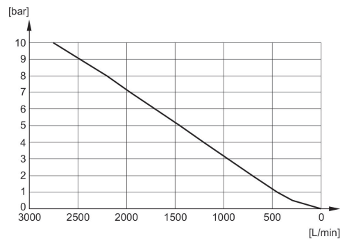
Flow diagram 1827000034
