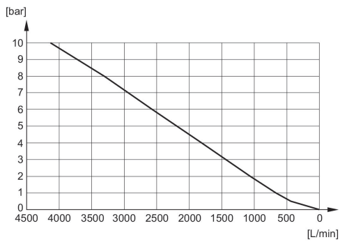
Flow diagram 1827000035
