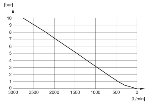
Flow diagram 1827000034
