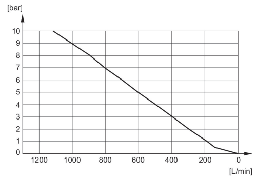
Flow diagram 1827000031
