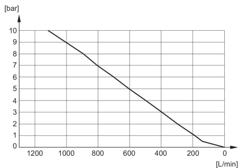
Flow diagram 1827000031
