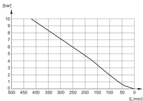
Flow diagram 1827000032
