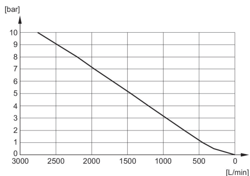
Flow diagram 1827000034
