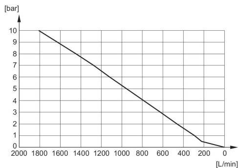
Flow diagram 1827000033
