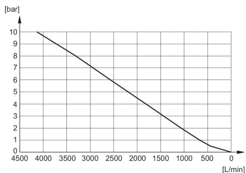
Flow diagram 1827000035
