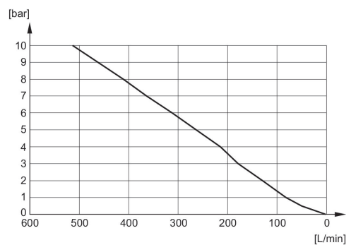
Flow diagram 1827430004
