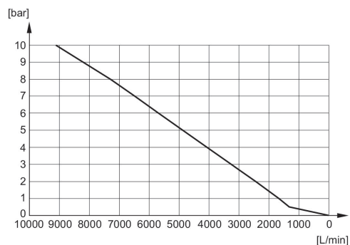
Flow diagram 1827000021
