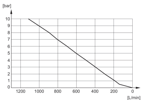
Flow diagram 1827000031
