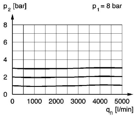
p_1 = Working pressure p_2 = Secondary pressure q_n = Nominal flow p_2 = 0,1 - 3 bar
