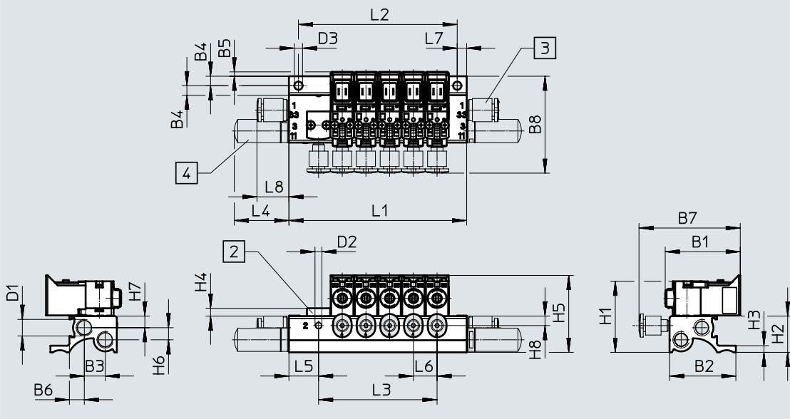
[2] Cover plate MHAP1
