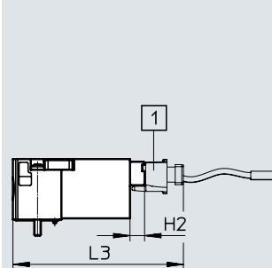
Plug connection at the rear
