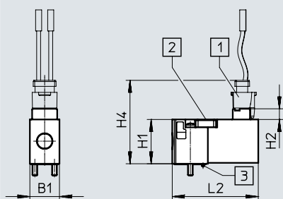
Plug connection on top
