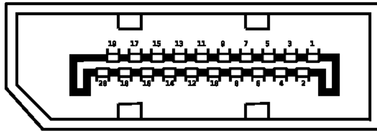
Figure 18: Disaply Port Connector
