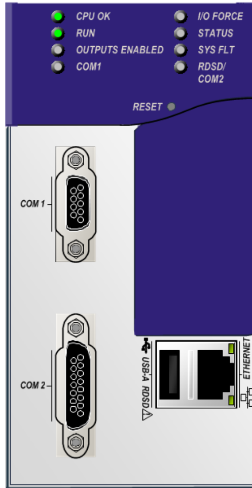
Figure 26: IC695CPE310 Front View
