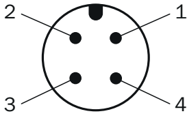
Pin assignment A (type S)
