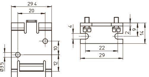
Fig. 3 Left wall mounting, right mounting bracket
