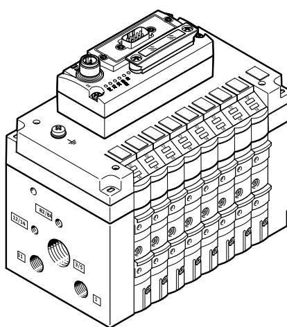
CPV valve terminal with I-Port interface with bus node
