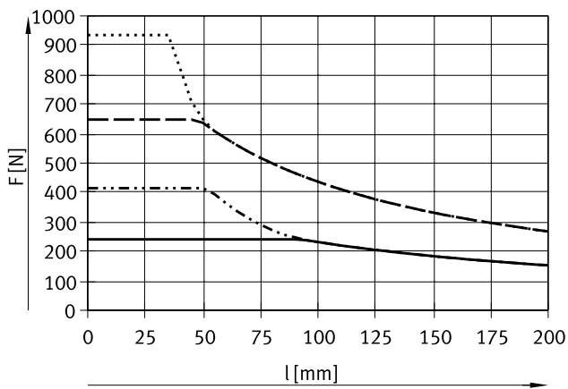
DFM-32 ... 63-KF, stroke 125 ... 200 mm
