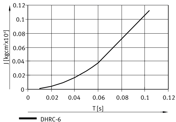
Opening and closing times T to be set at 0.6 MPa (6 bar, 87 psi) as a function of mass moment of inertia of the gripper fingers – DHRC-6
